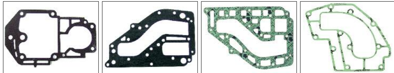
S610485012010 EXHAUST GASKET 61T-45113-A0 S610485012011 EXHAUST GASKET 6K8-41124-A1 S610485012012 EXHAUST GASKET 6K8-41122-A1 S610485012013 EXHAUST GASKET 6K8-41114-A1
