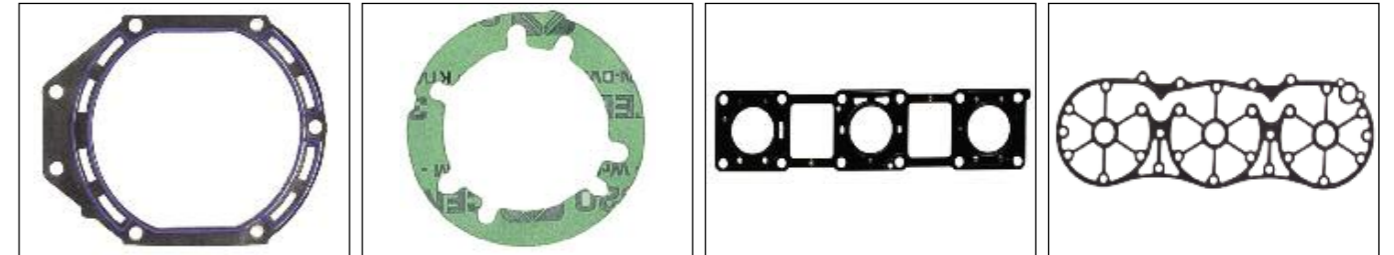
S610485012032 EXHAUST GASKET 64X-41124-00 S610485012033 EXHAUST GASKET 64X-14623-00 S610485012034 EXHAUST MANIFOLD GASKET 66V-14613-01 S610485012035 EXHAUST MANIFOLD GASKET 66V-11193-01
