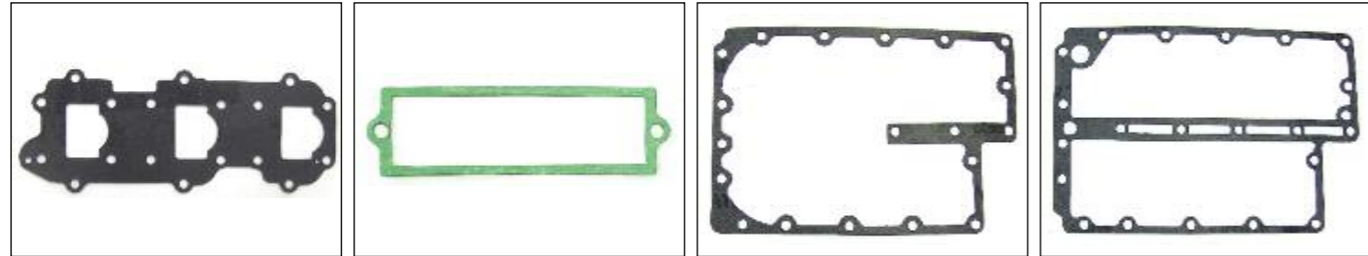
S610245010017 REED GASKET 317305 S610245010018 REED GASKET 332266 S610245012001 EXHAUST PLATE GASKET 317955 S610245012002 EXHAUST COVER GASKET 317914
