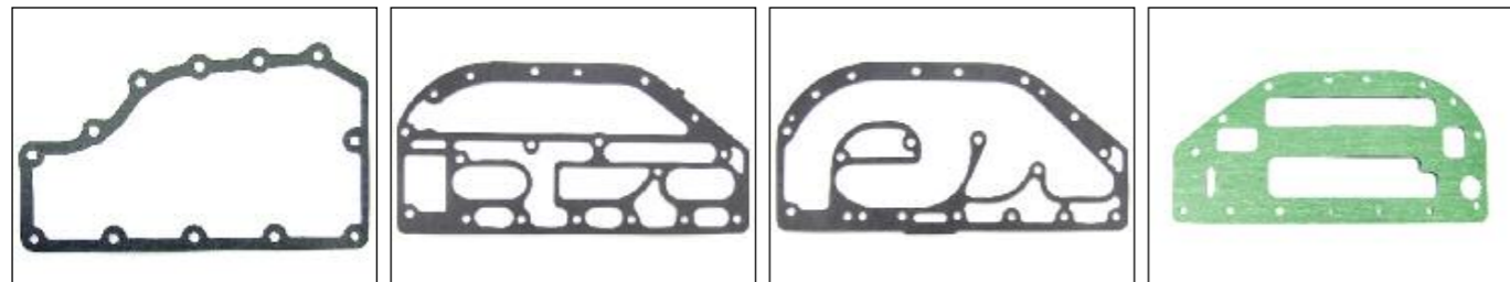
S610245012009 EXHAUST COVER GASKET 325211 S610245012010 INNER EXHAUST GASKET 331917 S610245012011 EXHAUST COVER GASKET 331916 S610245012012 EXHAUST COVER GASKET 329833
