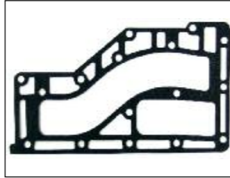
S610485012079 GASKET EXHAUST OUTER 6E9-41114-A0
