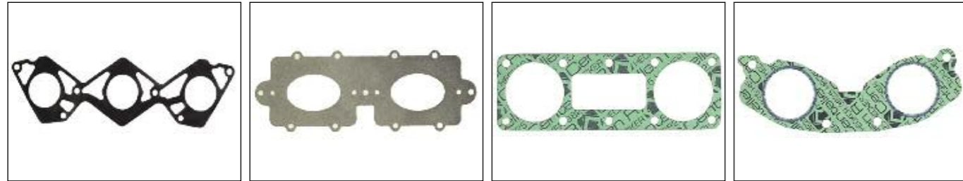
S610485010015 INTAKE MANIFOLD GASKET 65U-13556-00 S610485010017 INTAKE MANIFOLD GASKET 39X-13621-01 S610485010018 INTAKE MANIFOLD GASKET 64X-13674-00 S610485010019 INTAKE MANIFOLD GASKET 64X-13556-00
