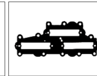
S610334010012 CARBURETOR GASKET 27-819113
