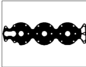
S610485015006 HEAD COVERGASKET 688-11193-01-00
