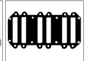
S610334047040 REED BLOCK GASKET 27-12775-5
